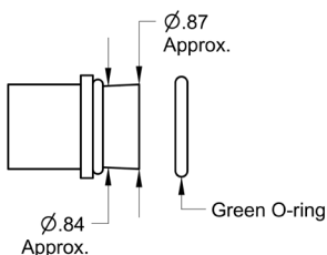
Tapered End
