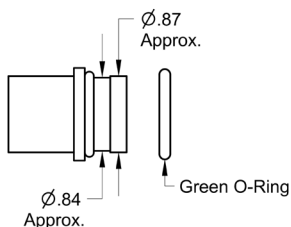
O-Ring Groove End
