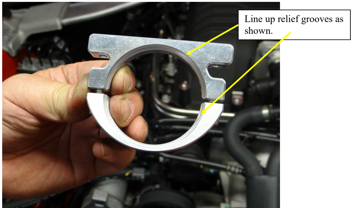
Step 6: Assemble billet saddle to billet clamp using (2) 1/4x20x5/8 SHCS do not tighten.
