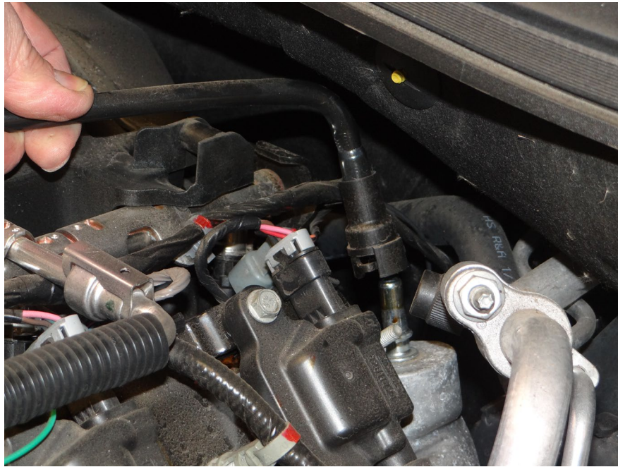
Step 4: Remove PCV line from valve cover.
